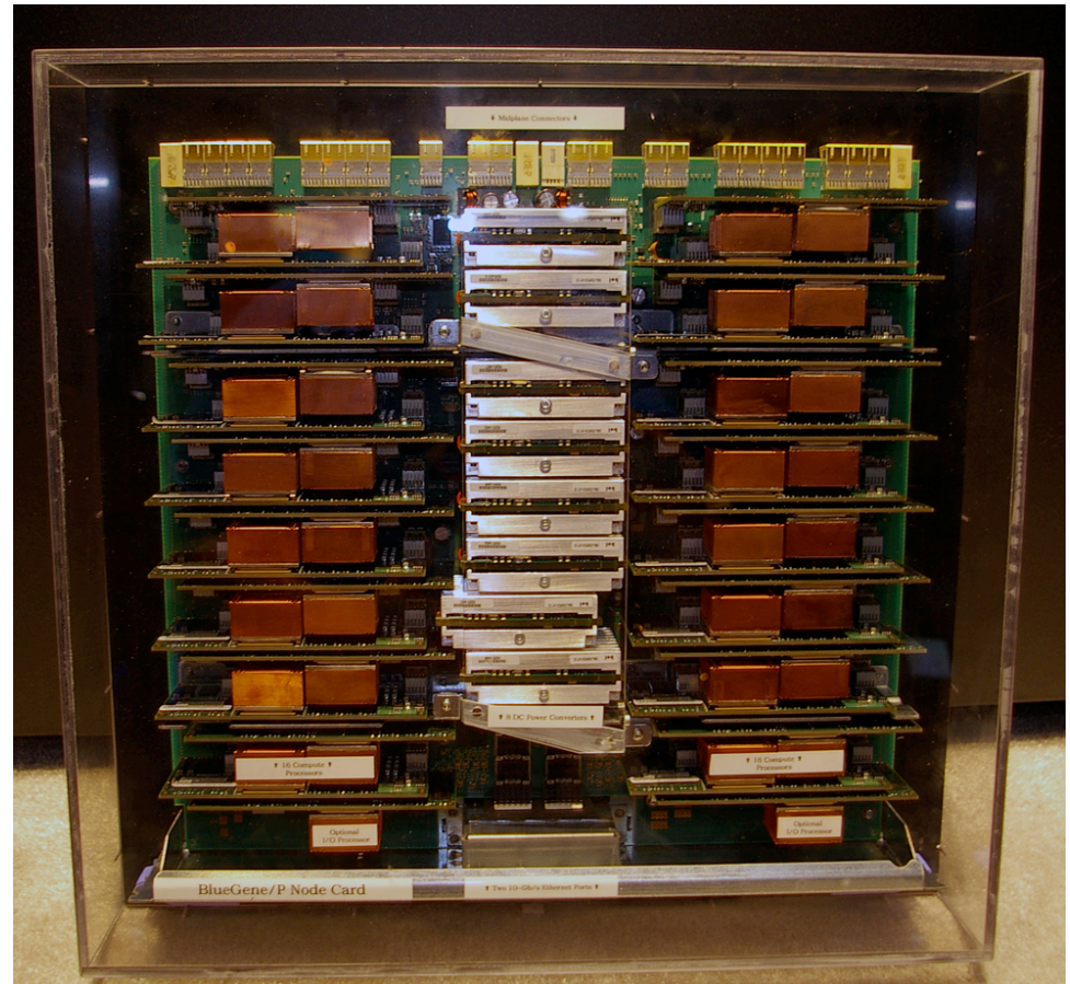
Blue Gene/P Node Card Prototype 32 Compute Processors 2 I/O Processors 2 10-Gb/s Ethernet Ports
