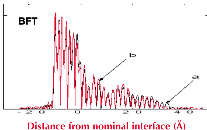
FIG. 1. Back Fourier transform of the complex structure factor of a 30-Å-thick \text{Gd}_2\text{O}_3 passivation layer on (100) GaAs. Note the non-monotonic variations in the electron density to the right of the interface. The two curves (a) and (b) correspond to different starting models for the structure, illustrating that the final best fit BFT is relatively insensitive to the details of the initial reference model.
