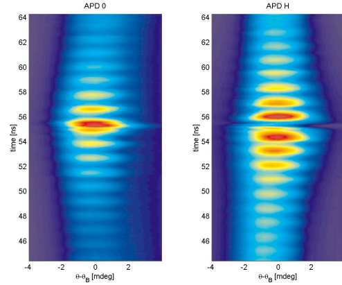
FIG. 2. Time-resolved Ge 20-2 rocking curve, when strain arrives at the exit face of crystal.
