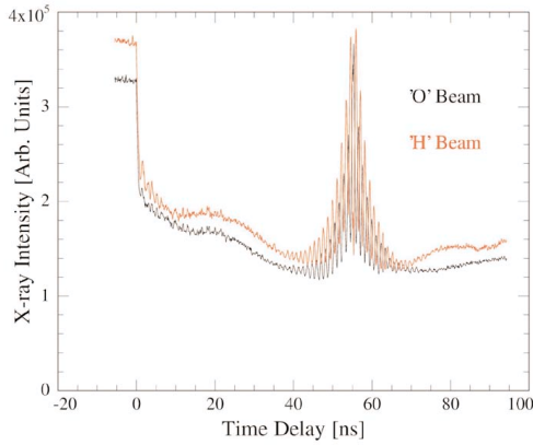
FIG. 1. Time-resolved x-ray diffraction following laser-induced strain in Ge 20-2.
